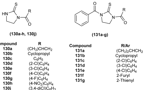
Fig. 58 Mono and di-acylated imidazolidine-2-thione derivatives.
