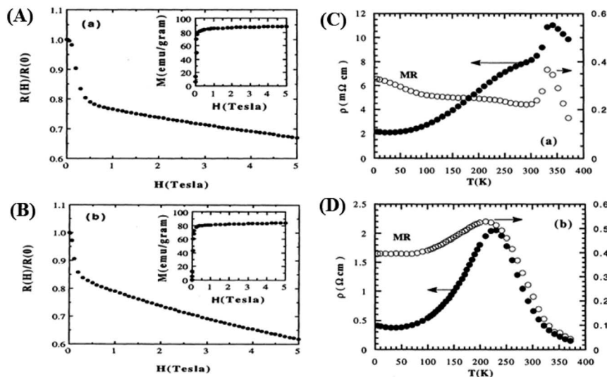
Fig. 2 [A] Field dependence of relative resistivity and magnetization at 5 K for, \text{La}_{0.67}\text{Ba}_{0.33}\text{MnO}_{2.99} and [B] \text{La}_{0.67}\text{Ba}_{0.33}\text{MnO}_{2.90} . Reprinted with permission from the American Physical Society. 54 Curves of resistivity (filled circles) and MR ratio (empty circles) against temperature for [C] \text{La}_{0.67}\text{Ba}_{0.33}\text{MnO}_{2.99} and [D] \text{La}_{0.67}\text{Ba}_{0.33}\text{MnO}_{2.90} . Reprinted with permission from the American Physical Society. 54
