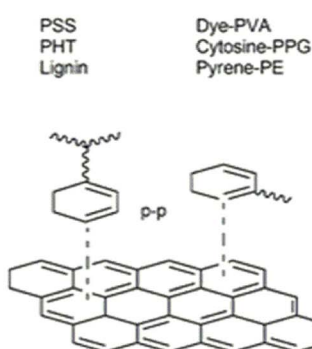
Fig. 20 Crystalline graphite powder with an aqueous solution of PVP under sonication which resulted in water-soluble polymer-protected graphene single layer. (a) CH- \pi bonding under polyethylene (PE), polyvinylpyrrolidone (PVP) polyvinylchloride (PVC), cellulose, chitosan and pullulan treatment, (b) \pi - \pi stacking (under poly(3,4-ethylenedioxythiophene) (PSS), polyhexahydrotriazine (PHT), lignin, dye-polyvinyl alcohol (dye-PVA), cytosine-polypropylene glycol (cytosine-PPG) and pyrene-polyethylene (pyrene-PE) treatment and (c) cation- \pi interaction.
