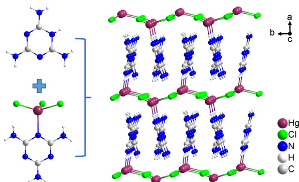
Fig. 9 Crystal structure of (\text{C}_3\text{N}_6\text{H}_7)(\text{C}_3\text{N}_6\text{H}_6)\text{HgCl}_3 .
