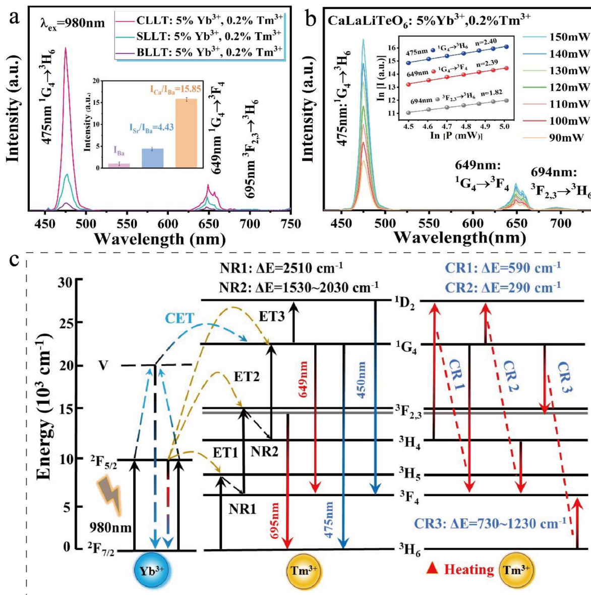
Fig. 3 (a) Up-conversion PL spectra of \text{ALaLiTeO}_6:5\% \text{Yb}^{3+}, 0.2\% \text{Tm}^{3+} ( A = \text{Ca}, \text{Sr}, \text{and Ba} ). (b) The relationship between \ln(I) and \ln(P) of \text{CaLaLiTeO}_6:5\% \text{Yb}^{3+}, 0.2\% \text{Tm}^{3+} . (c) Energy level diagram and thermally enhanced CR processes in the \text{ALaLiTeO}_6:5\% \text{Yb}^{3+}, 0.2\% \text{Tm}^{3+} phosphor.
