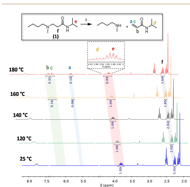
Fig. 2 ^1\text{H} NMR stacking spectra of model compound 1 in DMSO- d_6 at 25 °C, 120 °C, 140 °C, 160 °C and 180 °C for 16 h.
