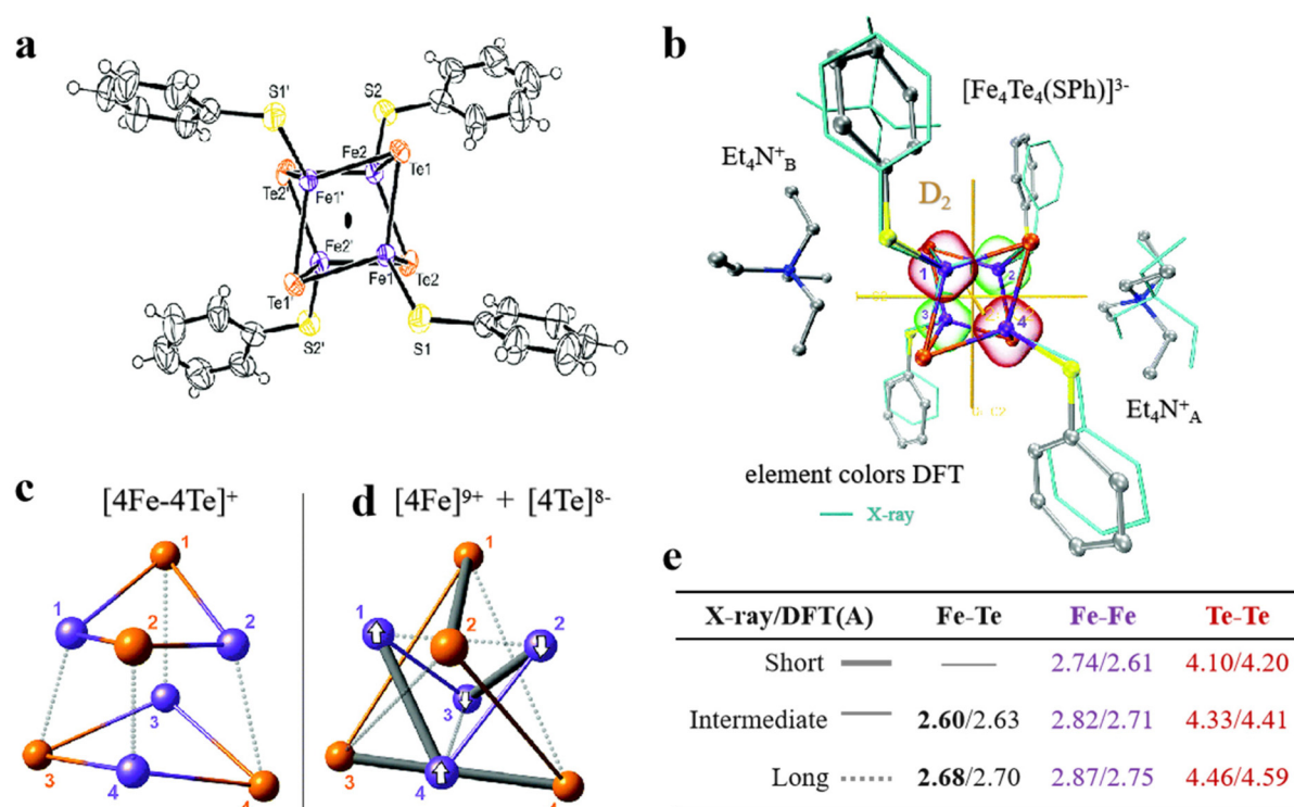
Fig. 9 Artificial Fe-S clusters based on Te element doping. (a) The structure of [Fe 4 Te 4 ] cluster. (b) D 2 -symmetric [Fe 4 Te 4 ] clusters obtained by X-ray and DFT optimization. (c and d) The bonding interactions and (e) bond length information of [Fe 4 Te 4 ] cluster cores. Reproduced with permission from ref. 98. Copyright 2019, Royal Society of Chemistry.
