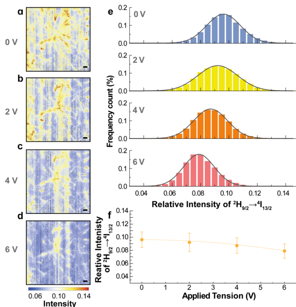
Fig. 6 (a–d) Maps showing the relative intensity of the ^2\text{H}_{9/2} \rightarrow ^4\text{I}_{13/2} transition in a selected region of the HSM images at increasing applied voltages. Corresponding mean temperatures are 297.1 K, 302.0 K, 318.5 K and 342.8 K, respectively. Scale bars are 5 \mu\text{m} . (e) Statistical analysis of the constructed maps. (f) Mean values of the relative intensity of the ^2\text{H}_{9/2} \rightarrow ^4\text{I}_{13/2} transition. The standard deviations are plotted as error bars.
