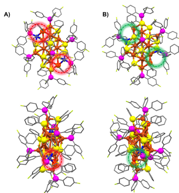
Fig. 1 The total structures of (A) Cu 22 -1 and (B) Cu 22 -2 from different views. Color labels: Cu = brown/blue, Se = yellow/red, P = purple, F = chartreuse, C = gray. For clarity, H atoms are omitted.
