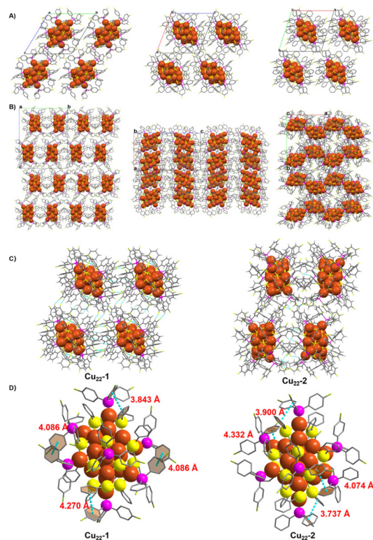
Fig. 3 Views of the assembled packing of (A) \text{Cu}_{22-1} and (B) \text{Cu}_{22-2} viewed along the a , b and c axes. (C) The intermolecular forces of C–F...H–C in the isomeric \text{Cu}_{22-1} and \text{Cu}_{22-2} . (D) The intramolecular forces of \pi\cdots\pi in the isomeric \text{Cu}_{22-1} and \text{Cu}_{22-2} . Cu = yellow, P = purple, F = chartreuse, C = gray. For clarity, H atoms are omitted.
