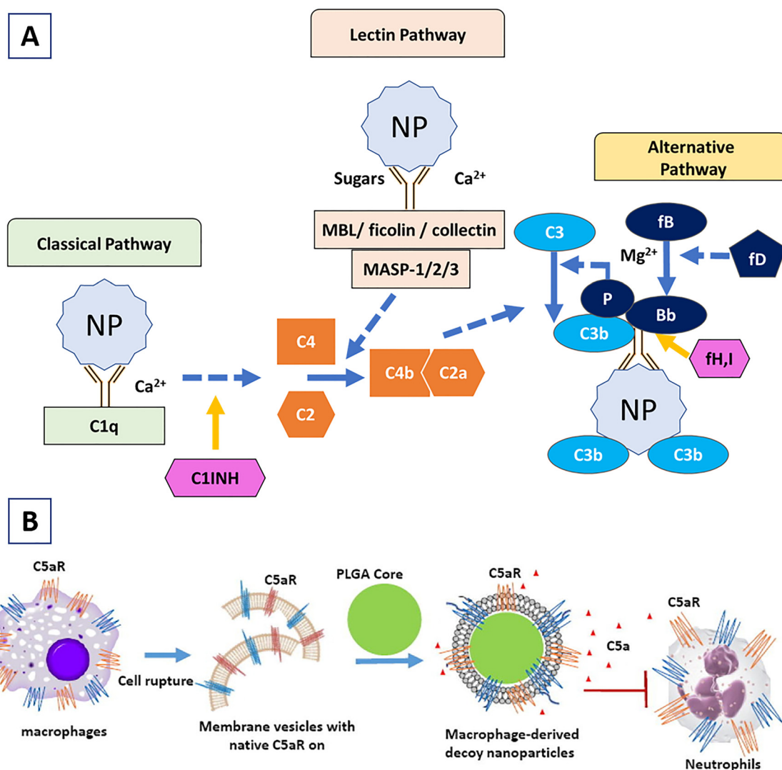
Fig. 9 (A) Schematic representation of the activation of the upstream part of the complement cascade through nanoparticle-bound immunoglobulins. The three initiating complement pathways include the classical, lectin and alternative pathway. The activation of the classical pathway occurs through C1q binding to the Fc portion of the surface-bound antibodies, the lectin pathway through the binding of the glycosylated regions of the antibodies to MBL/MASP-2 and the alternative pathway through the deposition of antibody-bound C3. The natural inhibitors of the complement cascade are shown in pink with yellow arrows. (B) Schematic illustration of the inhibition of neutrophil activation through C5aR-displaying decoy nanoparticles for improved mesenchymal stem cell-based therapies. Reproduced with permission from ref. 278. Copyright 2019, Elsevier. Abbreviations used: NP-nanoparticles; C1, C2, C3, C4-complement proteins; MBL-mannose-binding lectin; MASP-MBL-associated serine proteases; fB, fD, fI, fH: complement factors.
