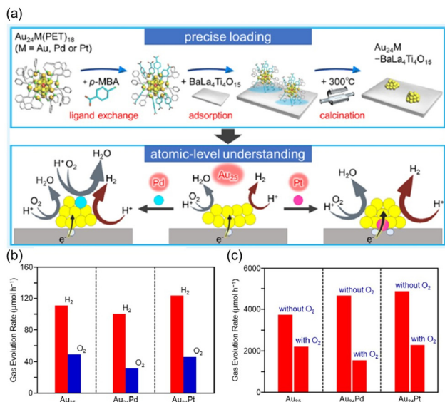
Fig. 5 (a) Schematic illustration of the synthesis procedure for the Au_{24}M/BaLa_4Ti_4O_{15} photocatalyst ( M = Au, Pd , or Pt ) and the role of the dopant in the HER. (b) Hydrogen and oxygen evolution rates for Au_{25} , Au_{24}Pd and Au_{24}Pt in photocatalytic water splitting under UV light. (c) Difference in the hydrogen evolution rate in the presence of methanol as a sacrificial reagent under a flow of Ar gas (without O_2 ) and a 7:3 mixture ratio of Ar to air (with O_2 ). Reproduced from ref. 49 with permission from the American Chemical Society, Copyright 2019.
