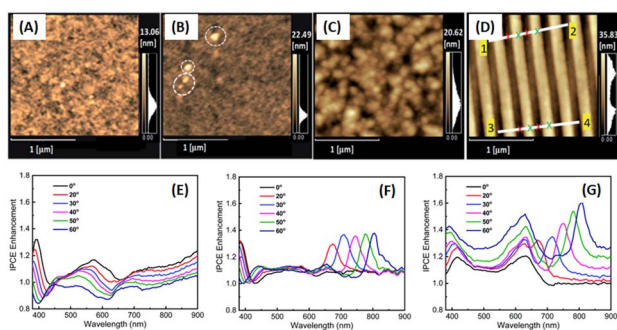
Fig. 24 AFM images of HTL films prepared from (A) PEDOS: PSS and (B) G-AuQD-loaded PEDOT: PSS. The white circles in (B) indicate the domains of aggregated G-AuQDs. AFM images of the (C) flat and (D) BD-R imprinted photoactive layers. (E–G) Spectra depicting the enhancement of IPCE for green-AuQD/BD-R OSCs under non-polarized light irradiation at different angles of incidence. The figures represent the IPCE enhancement spectra for (E) G-AuQD OSC, (F) BD-R OSC, and (G) G-AuQD/BD-R OSC. Reproduced from ref. 110 with permission from the Royal Society of Chemistry (CC BY-NC 4.0).
