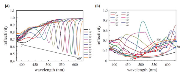
Fig. 25 SPR reflectivity curves for (A) AuQD films on a PEDOT: PSS layer deposited on a silver-deposited BD-R grating substrate and (B) AuQD films on a PEDOT: PSS layer deposited on a silver-deposited DVD-R grating substrate. Reproduced from ref. 109 with permission from the Royal Society (CC BY-NC 4.0).
