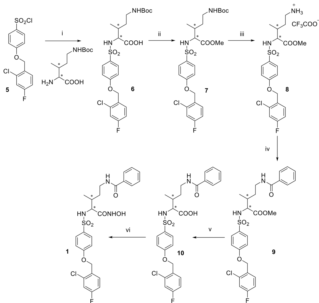
Scheme 1 Reagents and conditions: (i) Et 3 N, H 2 O/dioxane 1 : 1, rt, 16 h, 79%; (ii) CH 3 l, K 2 CO 3 , DMF dry, rt, 3 h, quantitative; (iii) TFA, DCM dry, rt, 3 h, 91%; (iv) benzoyl chloride, DIPEA, DMF dry, rt, 3 h, 99%; (v) LiOH 1 N, MeOH, 60 °C, 6 h, 75%; (vi) 1. THPONH 2 , EDC, HOBt, NMM, DMF dry, rt, 18 h; 2. HCl 4 N, MeOH/dioxane 1 : 1, rt, 6 h, 16% over two steps.
