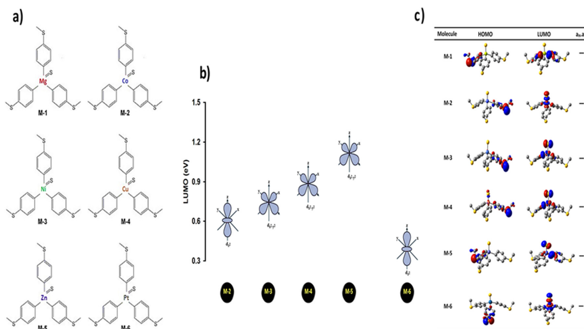
Fig. 1 (a) Schematic illustration of tripod connectors with six different metal centres; (b) schematic showing the d-orbital shape of some transition metals (Co, Ni, Cu, Zn, and Pt respectively); (c) optimized geometry of all the molecules in a gas phase, and their HOMOs and LUMOs (isosurfaces \pm 0.02 (e bohr −3 ) 1/2 ). The blue part is a positive sign, while the red part is a negative sign. a_H \cdot a_L is the multiplication of the HOMO and LUMO amplitudes. As an example, the HOMO and LUMO for the M-1 molecule possess different signs, and thus the multiplication of the molecular orbitals amplitudes ( a_H \cdot a_L ) is a negative sign and the molecule exhibits constructive quantum interference (CQI).
