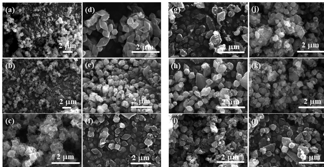
Fig. 6 SEM micrographs of MIL-88B(Fe) (a)–(f) and SAF7@MIL-88B(Fe) (g)–(i) after incubation in PBS (a)–(c) and (g)–(i) and RPMI (d)–(f) and (j)–(l) media for 24, 48 and 72 hours at 37 °C.
