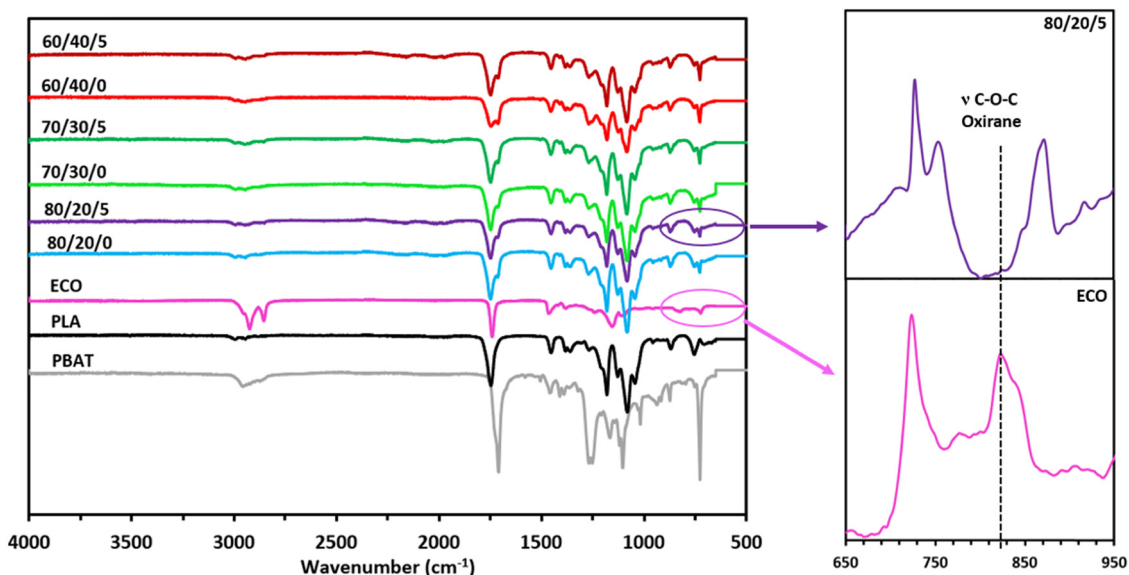
Fig. 1 FTIR spectra of neat polymers, ECO, and all PLA/PBAT blends.
