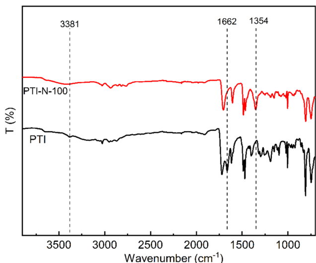
Fig. 3 FT-IR spectra of PTI and PTI-N-100.
