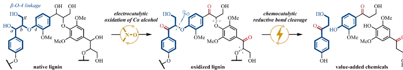
Fig. 2 Electrocatalytic oxidation of lignin model compound.
