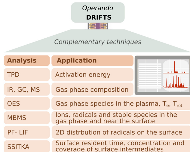
Fig. 3 Scheme highlighting analytical techniques complementary to operando DRIFTS: temperature-programmed desorption (TPD), infrared (IR) or mass spectrometry (MS), optical emission spectroscopy (OES), molecular beam mass spectrometry (MBMS), photofragmentation laser-induced fluorescence (PF-LIF), steady-state isotopic transient kinetic analysis (SSITKA).
