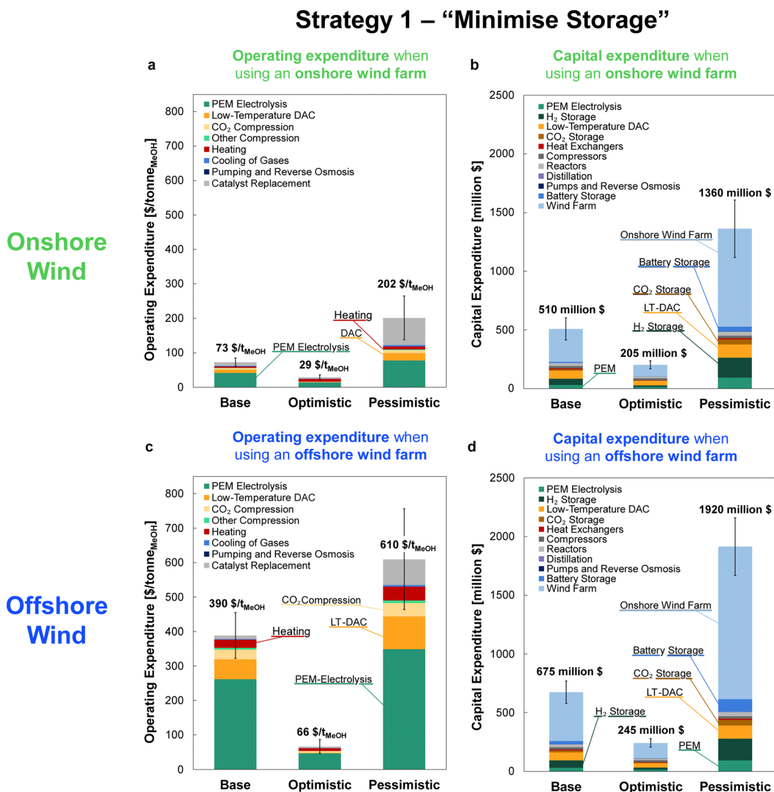
Fig. 9 The costs of methanol production via DAC-PtM, operating under Strategy 1 (“minimise storage”) for the three optimization cases: base, optimistic, and pessimistic. (a) The operating expenditure (OPEX) with an onshore wind farm. (b) The capital costs (CAPEX) when reliant on an onshore wind. (c) The OPEX with an offshore wind farm. (d) The CAPEX with an offshore wind farm. The contributions are stacked as ordered in the legend, starting with PEM electrolysis at the base. Significant contributions are also labelled on the graphs. Error bars are provided, according to the estimated uncertainty in model parameters, detailed in Section S11 (ESI † ).
