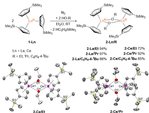
Fig. 2 Top: synthesis of 2-Ln/R by alcoholysis of 1-Ln in Et 2 O. Bottom: crystal structures of 2-Ce/Et and 2-Ce/iPr with displacement ellipsoids at the 50% probability level. Hydrogen atoms and disorder were removed for clarity.
