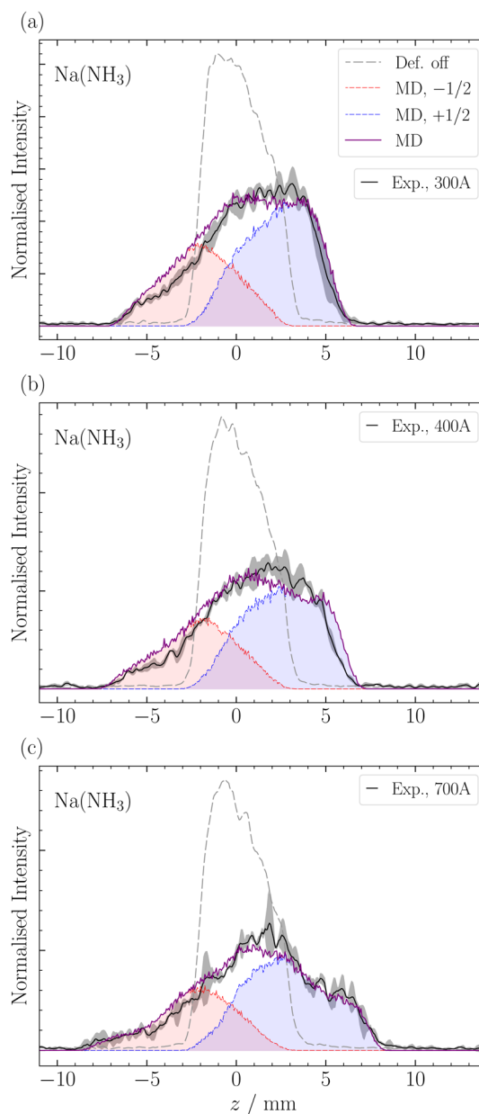
Fig. 4 Magnetic deflection of \text{Na}(\text{NH}_3) measured at a magnification of M_r = 1 and a current of 300 A, 400 A, and 700 A (a)–(c). The dashed grey and the black lines correspond to the experimental spatial distribution when the deflector is off and on, respectively. The purple line illustrates the total deflection obtained in our simulations, while the red and blue lines delineate the contributions of the two spin projections. Shaded areas represent experimental uncertainties at 1\sigma .
