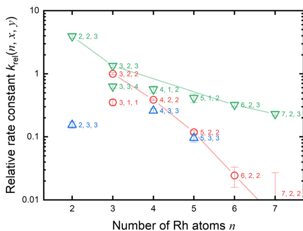
Fig. 6 Relative rate constant k_{\text{rel}}(n, x, y) of the reduction reaction of \text{Rh}_n\text{N}_x\text{O}_y^+ at 903 K was estimated by measuring the decreasing rate of the fraction of \text{Rh}_{3-7}\text{N}_2\text{O}_2^+ , \text{Rh}_{2,4}\text{N}_3\text{O}_3^+ , and \text{Rh}_n\text{N}_x\text{O}_{x+1}^+ with the CO concentration for each n . Rate constants were normalized to that of \text{Rh}_3\text{N}_2\text{O}_2^+ . Red circles, blue triangles, and green triangles correspond to \text{Rh}_n\text{N}_2\text{O}_2^+ , \text{Rh}_n\text{N}_3\text{O}_3^+ , and \text{Rh}_n\text{N}_x\text{O}_{x+1}^+ , respectively. To indicate the size-dependence of \text{Rh}_n\text{N}_2\text{O}_{2,3}^+ , the lines are shown as a guide.
