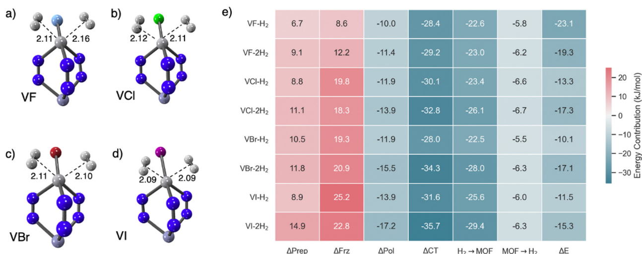
Fig. 13 Multiple \text{H}_2 ligations in V(II)-X-MFU-4l, (X = F, Cl, Br, I) (a)–(d) and EDA of the quite wide range of adsorption behaviour as a function of the halide counterion (e). Dative effects, particularly forward donation, dominate the binding energy. Distances are reported in Å, and energy contributions in \text{kJ mol}^{-1} in (e).
