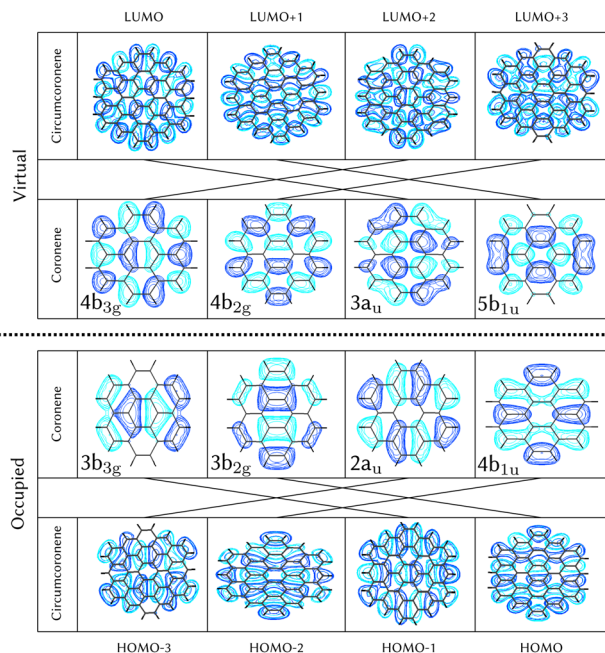
Fig. 3 Top view of molecular orbitals of circumcoronene showed in comparison with respect to the corresponding ones in coronene. All these orbitals correspond to \pi^* orbitals asymmetric with respect to the molecular plane. Symmetry labels are included for the coronene system, connected with lines with equivalent MO in circumcoronene, where the symmetry can be extrapolated.
