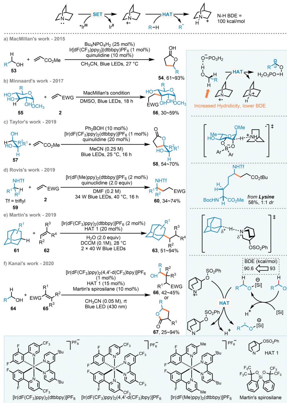
Scheme 21 Hydroalkylation of alkenes with various \text{C}(\text{sp}^3)\text{-H} bonds via quinclidines mediated HAT process.
