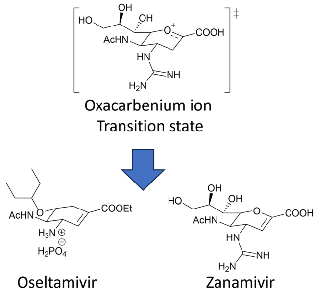
Fig. 17 Chemical structure of the two NA inhibitors, Osetamivir and Zanamivir, both mimic the oxocarbenium ion of the sialic acid intermediate formed during the NA action.
