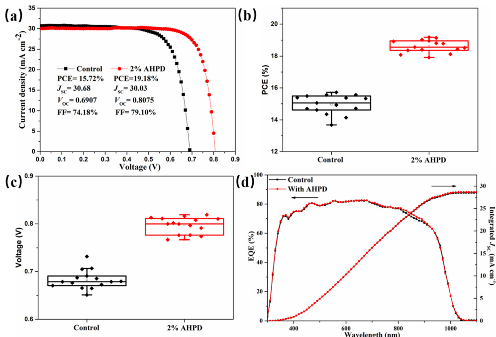
Fig. 4 (a) J - V curves of the champion AHPD-treated and control devices with a reverse scan. (b) PCE distribution of the control and AHPD-treated devices. (c) V_{\text{OC}} distribution of the control and AHPD-treated devices. (d) EQE spectra of the champion AHPD-treated and control devices, and the corresponding integrated J_{\text{SC}} curves.
