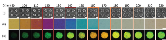
Fig. 6 SEM (i), reflected bright field (ii), and upconversion luminescence (iii) color patches of pixel arrays with D = 90\text{--}220 nm and s = 100 nm. 90
