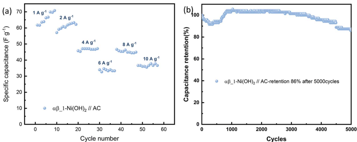
Fig. 11 (a) The specific capacitance evolution under various current densities of \alpha\beta\text{-1-Ni(OH)}_2 // \text{AC} . (b) Cycling performance at 100 \text{mA cm}^{-1} for 5000 cycles.
