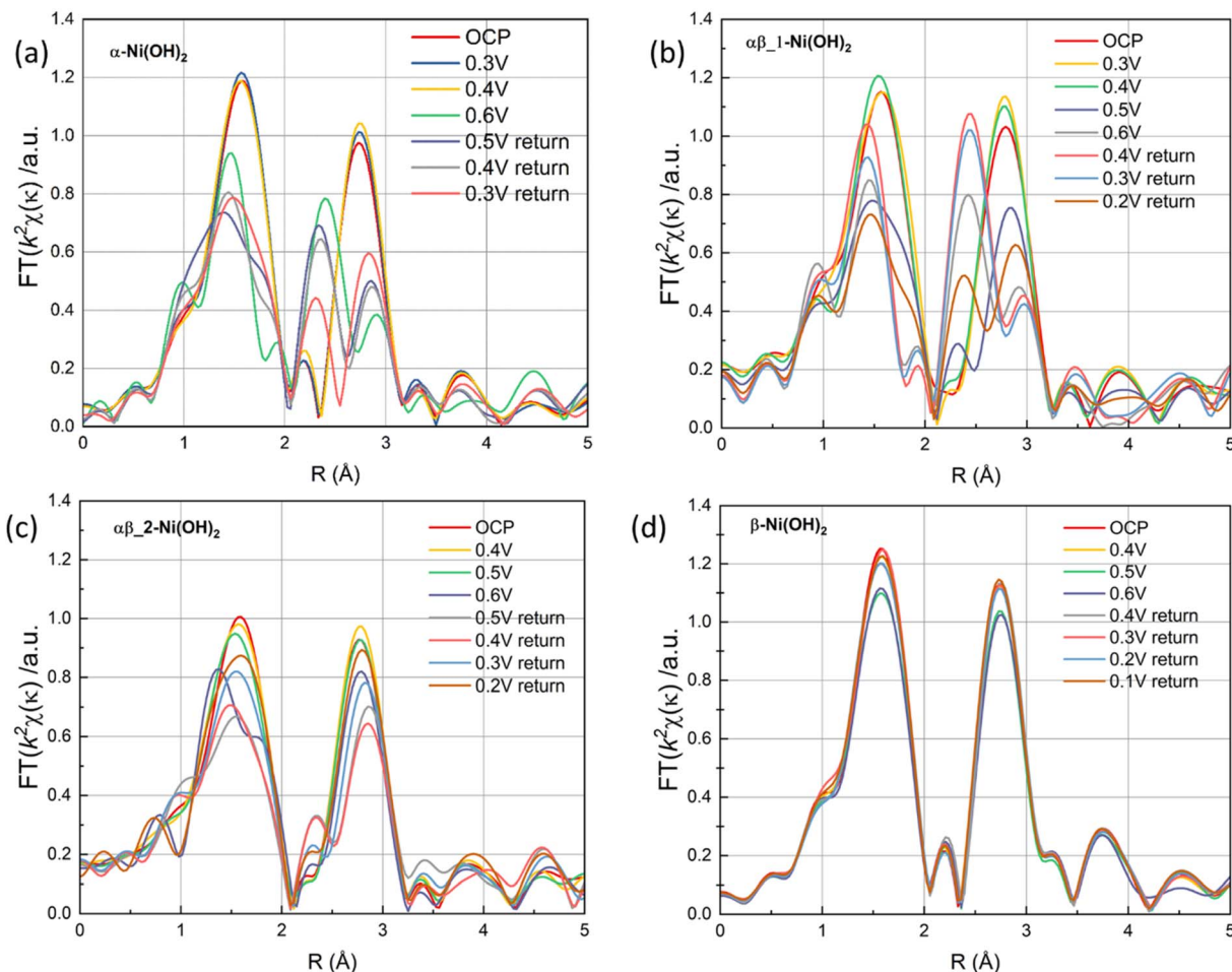
Fig. 10 The FT signal of the \kappa^2 -weighted EXAFS (a) \alpha\text{-Ni(OH)}_2 , (b) \alpha\beta\text{-1-Ni(OH)}_2 , (c) \alpha\beta\text{-2-Ni(OH)}_2 and (d) \beta\text{-Ni(OH)}_2 under a oxidation and reduction scans.
