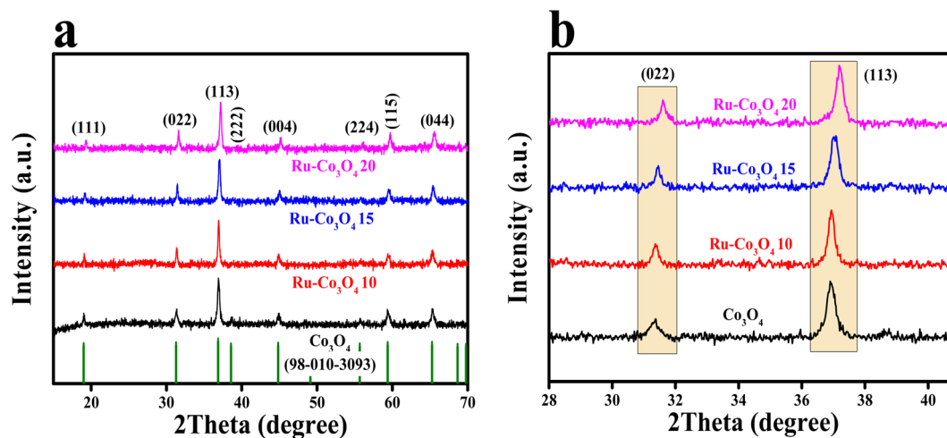
Fig. 1 (a) PXRD patterns of Co-BTC derived \text{Co}_3\text{O}_4 , Ru- \text{Co}_3\text{O}_4 10, Ru- \text{Co}_3\text{O}_4 15 and Ru- \text{Co}_3\text{O}_4 20; (b) enlarged PXRD pattern of (022) and (113) planes.
