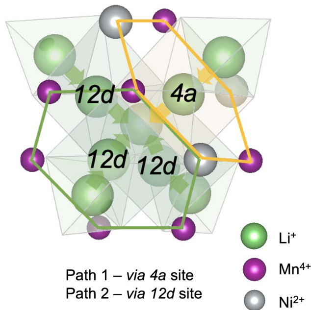
Fig. 10 A schematic showing 4a and 12d gate sites giving two distinct Li + migration paths in P 4/3 32 LiMn 1.5 Ni 0.5 O 4 . The 4a site surrounded by 3Mn 4+ and 3Ni 2+ ; the 12d sites surrounded by 5Mn 4+ and a Ni 2+ . Path 1 and path 2 are denoted by yellow and green arrows, respectively. Oxygen atoms which define the polyhedral vertices are not shown for clarity.
