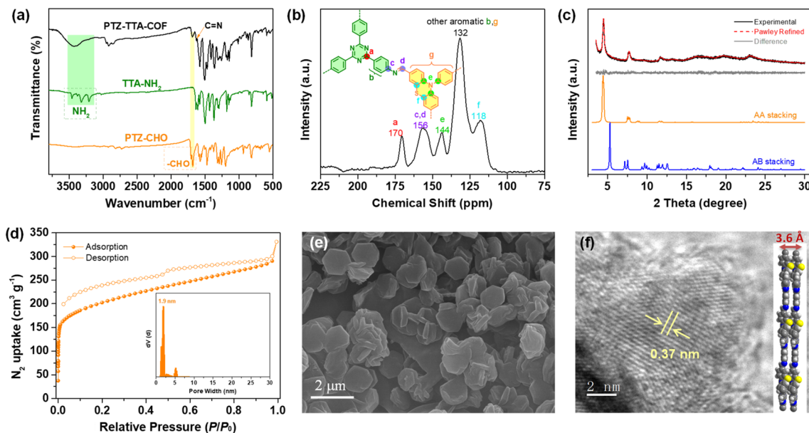
Fig. 2 (a) FT-IR spectra of PTZ-CHO, TTA-NH 2 and the PTZ-TTA-COF. (b) Solid-state 13 C CP-MAS NMR of the PTZ-TTA-COF. (c) Experimental PXR D, Pawley refinement and the difference of the PTZ-TTA-COF, and their simulated PXR D profiles in AA and AB stacking modes. (d) Nitrogen sorption isotherm of the PTZ-TTA-COF at 77 K; inset: pore size distribution derived from the QSDFT model. (e) SEM and (f) HR-TEM images of the PTZ-TTA-COF.
