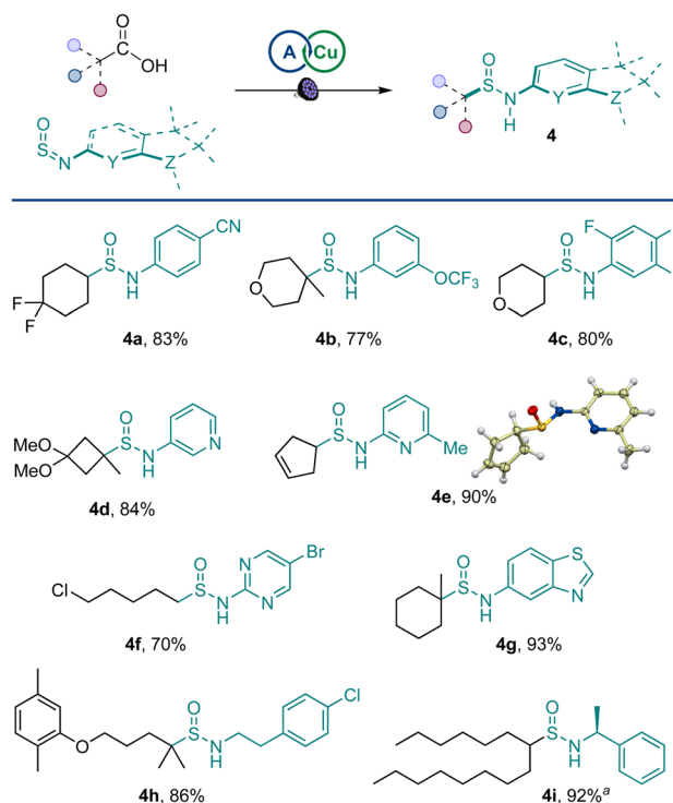
Scheme 2 Scope of sulfinylamines. Reaction conditions: carboxylic acid (0.2 mmol), sulfinylamine (from the corresponding amine by activation with thionyl chloride, 0.4 mmol), A1 (10 mol%), Cu(MeCN) 4 BF 4 (3 mol%), dtbpy (4 mol%), CH 2 Cl 2 /MeCN (2 : 1, 2 mL), LED light (400 nm), 16 h. a 1 : 1 dr.
