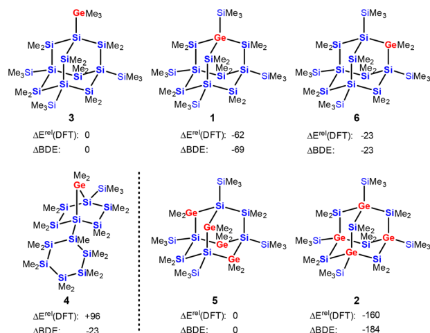
Fig. 3 Relative energies \Delta E^{\text{rel}} (DFT), in \text{kJ mol}^{-1} , of selected \text{Si}_{13}\text{Ge}_1\text{Me}_{24} and \text{Si}_{10}\text{Ge}_4\text{Me}_{24} isomers. Both calculated at M06-2X/6-311+G(d,p) and estimated on the basis of bond dissociation energies \Delta \text{BDE} .
