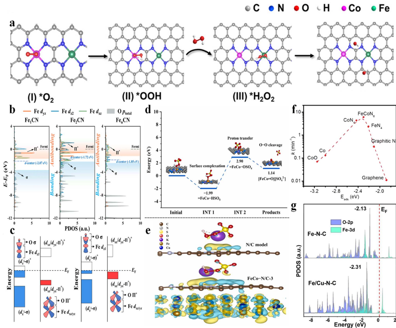
Fig. 2 (a) (I–IV) Proposed mechanism of \text{O}^{\bullet}\text{H} electro-generation from the ORR on \text{Co-N}_4/\text{Fe-N}_4(\text{CoFe}) , with permission from ref. 3 copyright 2023 ACS. (b) Projected density of states (PDOS) for \text{Fe-3d}_{yz}/d_{z^2}/d_{xz} orbitals and \text{O-p} orbitals of adsorbed PMS, with permission from ref. 9 copyright 2022 ACS. (c) Schematic illustration of the orbital interaction between \text{Fe-3d} ( d_{z^2} and d_{xz}/d_{yz} ) and \text{O} ( \sigma and \pi ) of adsorbed PMS ( \text{II}^* and \sigma ) of \text{Fe} sites in \text{Fe}_1\text{CN} and \text{Fe}_2\text{CN} , with permission from ref. 9 copyright 2022 ACS. (d) Potential energy profiles of the pathway for the generation of high-valent metal-oxo species, with permission from ref. 10 copyright 2022 Elsevier. (e) The calculated charge density difference diagrams of PMS adsorbed on the N/C model and \text{FeCo-N/C-3} . Isosurface contour is 0.0003e per \text{bohr}^3 . The light yellow and light blue correspond to the electron accumulation and electron depletion, respectively, with permission from ref. 10 copyright 2022 Elsevier. (f) Volcano plot of the reaction rate as a function of E_{\text{ads}} of PMS at various active sites, with permission from ref. 7 copyright 2021 Elsevier. (g) PDOS values calculated for the O-2p and Fe-3d orbitals in \text{Fe-N-C} and \text{Fe/Cu-N-C} , with permission from ref. 13 copyright 2022 Elsevier.
