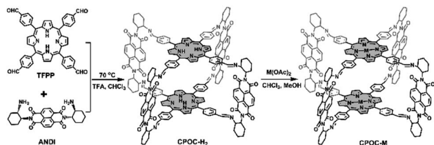
Scheme 1 Schematic synthesis of CPOC-M ( M = \text{H}_2 , \text{Co(II)} , \text{Ni(II)} , \text{Cu(II)} , \text{Zn(II)} ).
