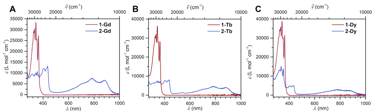
Fig. 2 Superimposed UV-vis spectra of [Cp* 2 Ln](μ-Bbim) ( 1-Ln , in red), and [K(crypt-222)][Cp* 2 Ln](μ-Bbim • ) ( 2-Ln , in blue), taken in THF. Concentrations: (A) 1-Gd : 2.636 \times 10^{-5} mol L −1 , 2-Gd : 3.198 \times 10^{-5} mol L −1 . (B) 1-Tb : 1.389 \times 10^{-5} mol L −1 , 2-Tb : 2.307 \times 10^{-5} mol L −1 . (C) 1-Dy : 1.353 \times 10^{-5} mol L −1 , 2-Dy : 1.114 \times 10^{-4} mol L −1 .
