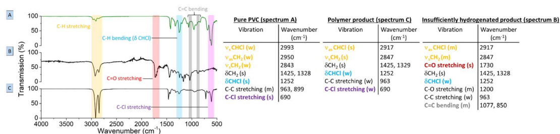
Fig. 3 ATR FTIR spectra and assignments of vibrational peaks. (A) PVC before reaction; (B) black precipitate formed after reaction with insufficient hydrogenation: significant \text{C=O} stretching and \text{C=C} bending peaks and char formation, indicated by a non-zero baseline (product obtained using 3.5 eq. of \text{Bu}_4\text{PbCl} , 2 mol% \text{H(CO)Rh(PPh}_3)_3 , in cyclohexanone at 180 °C for 2 h); (C) yellow product from effective tandem dehydrochlorination-hydrogenation, with intense \text{C-H} stretching vibrations and weakened \text{C-Cl} stretching vibrations (product obtained using 0.85 eq. of \text{Bu}_4\text{PbCl} , butanone and 2 mol% \text{H(CO)Rh(PPh}_3)_3 at 180 °C).
