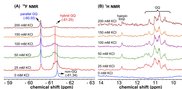
Fig. 6 (A) ^{19}\text{F} NMR and (B) ^1\text{H} NMR spectra of TFBF-modified ON 4 at different KCl concentrations.
