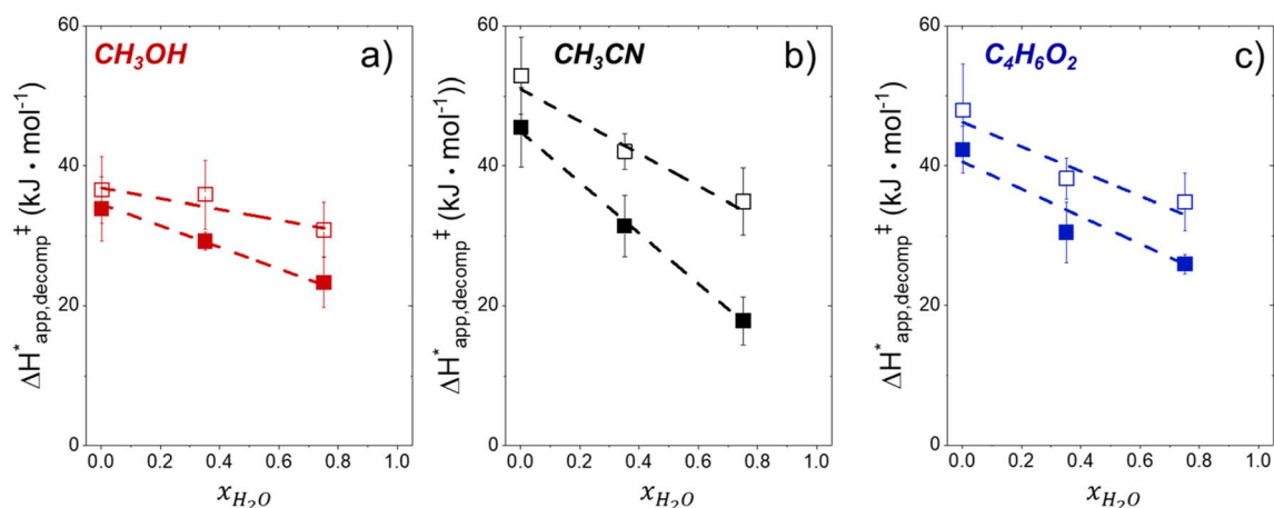
Fig. 6 \Delta H^*_{app,decomp} values for H_2O_2 decomposition (1 mM H_2O_2 , 313–343 K) as a function of x_{H_2O} in mixtures of (a) CH_3OH (■, □), (b) CH_3CN (■, □), and (c) C_4H_6O_2 (■, □) with H_2O over Ti-BEA-OH (solid) and Ti-BEA-F (hollow).
