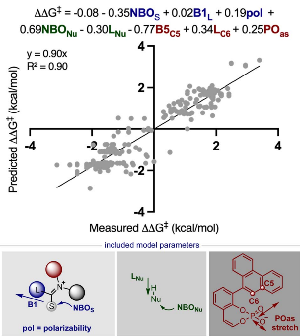
Fig. 4 The published statistical model describing the chiral phosphate catalysed nucleophilic addition to iminium intermediates. 'NBOs' and 'NBO Nu ' are the natural bond orbital parameters corresponding to the first atom of the iminium small group (usually a hydrogen) and the nucleophilic site (either a carbon, hydrogen, oxygen, or nitrogen), 'B1 L ' is the minimum width (Sterimol B1) of the largest iminium substituent, 'pol' is the calculated polarizability of the iminium, 'L Nu ' is the nucleophile length (Sterimol L), B5 C5 is the maximum width (Sterimol B5) of the catalyst 5-substituent, L C6 is the length of the catalyst 6-substituent, and finally 'PO as ' is the asymmetric P–O stretching frequency.
