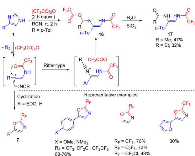
Scheme 13 Formation of bis(enamides) 17 and oxazoles 7 by the cleavage of NH-1,2,3-triazoles with trifluoroacetic anhydride in nitrile solvent.
