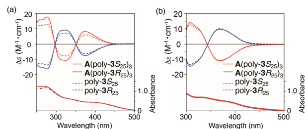
Fig. 6 CD and absorption spectra of optically active star polymers A (poly- 3S 25 ) 3 and A (poly- 3R 25 ) 3 and the corresponding linear polymers (poly- 3S 25 and poly- 3R 25 ) in THF at −10 °C (a) and in toluene at −10 °C (b).
