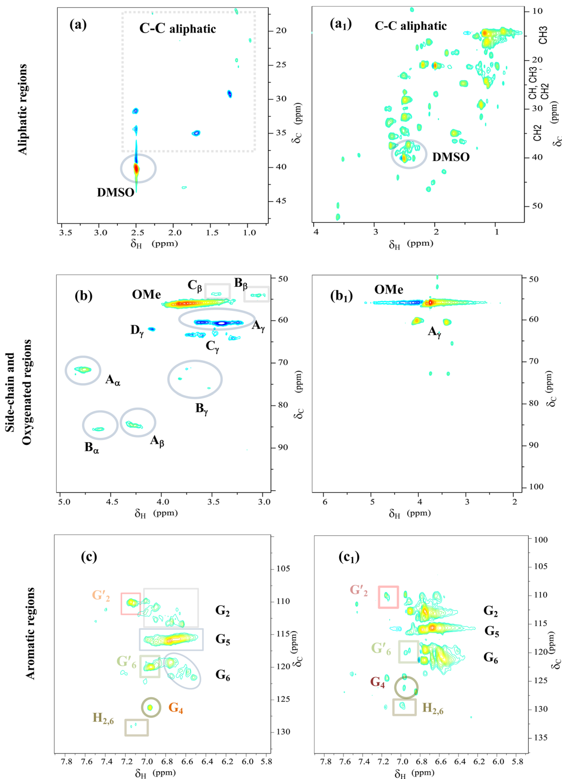
Fig. 9 2D HSQC NMR spectra of Kraft lignin (a, b and c) and light-oil (a 1 , b 1 and c 1 ) obtained at 290 °C for 4 h over CoMo/SBA-15 catalyst.
