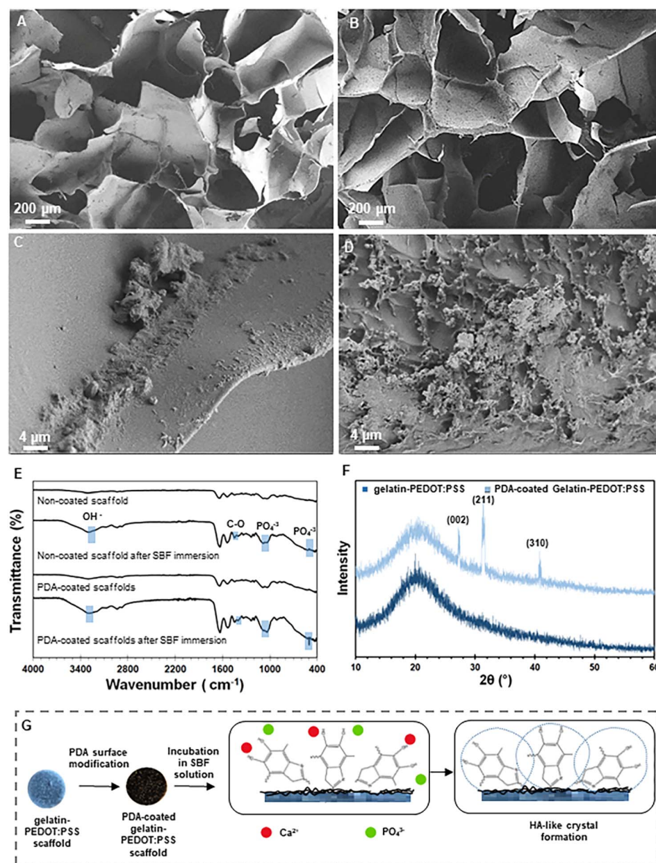
Fig. 4 Bioactivity of the constructs. (A–D) FE-SEM micrographs ((A, C) gelatin-PEDOT:PSS and (B, D) PDA-coated gelatin-PEDOT:PSS scaffolds), (E) FTIR spectra and (F) XRD patterns of mineralized HA-like layer on the surface of PDA modified and unmodified scaffolds after 4 weeks of immersion in SBF solution. (G) Representation of bioactivity mechanism.
