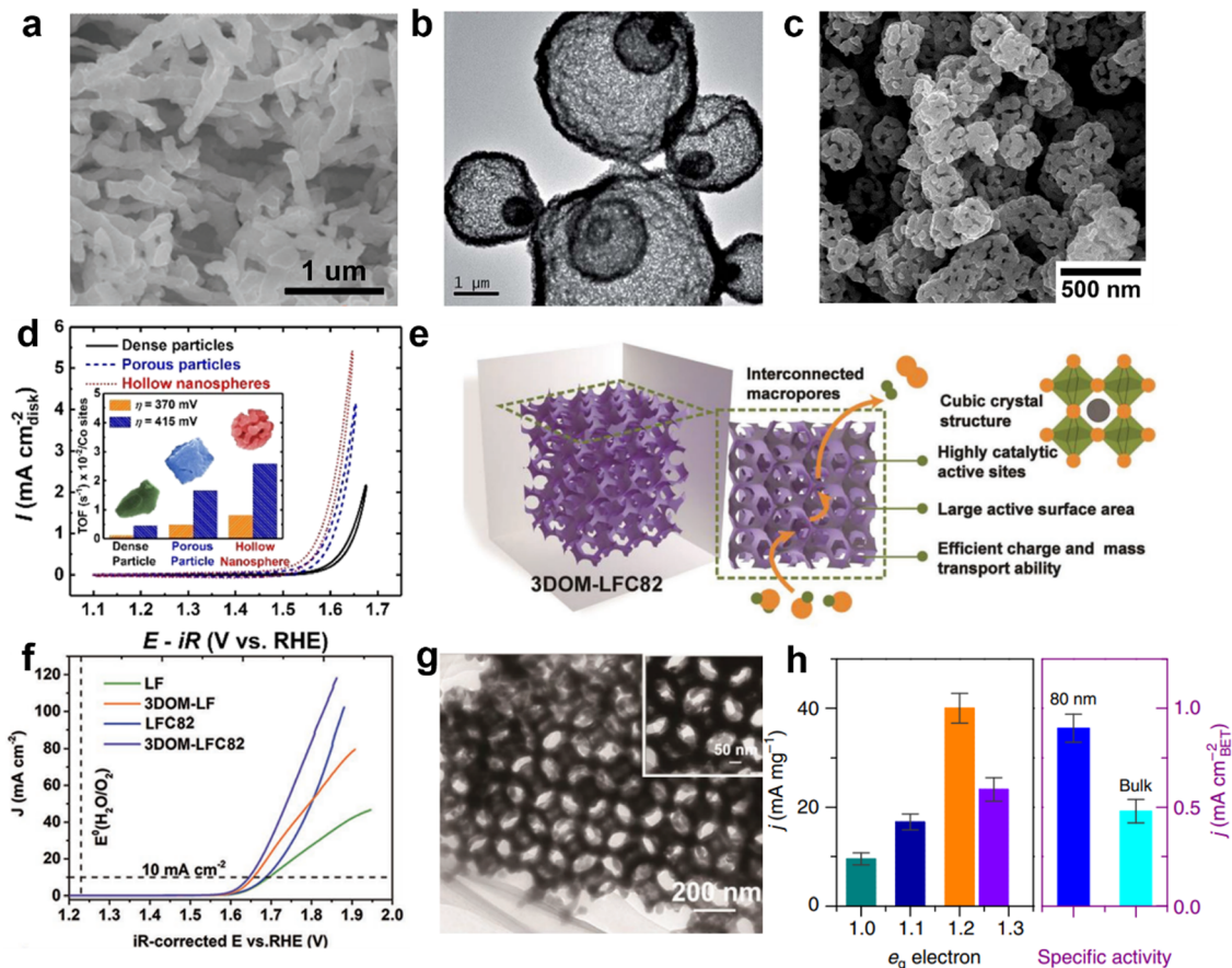
Fig. 8 (a) Scanning electron microscopy (SEM) image of nanorods SrNb 0.1 Co 0.7 Fe 0.2 O 3-δ prepared by electrospinning technology. Reproduced with permission. 91 Copyright 2016 WILEY-VCH Verlag GmbH & Co. KGaA, Weinhei. (b) TEM image of Yolk-Shell La 0.9 Sr 0.1 CoO 3 . Reproduced with permission. 92 Copyright 2015, The Royal Society of Chemistry. (c) SEM images of hollow spheres LaCoO 3 . (d) CV curves of LaCoO 3 with different morphologies for the OER. Reproduced with permission. 93 Copyright 2017, American Chemical Society. (e) Schematic diagram of the advantages of 3D ordered macro-porous electrocatalysts for the OER. (f) LSV curves of various catalysts for the OER. (g) TEM image for 3D ordered macro-porous electrocatalysts. Reproduced with permission. 94 Copyright 2018, WILEY-VCH Verlag GmbH & Co. KGaA, Weinheim. (h) Mass and special activities for nanoparticle catalysts of different sizes at an overpotential = 0.49 V. Reproduced with permission. 95 Copyright 2016, Springer Nature.
