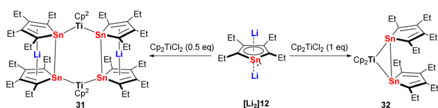
Scheme 5 Reaction of tetraethyldilithiostannole [\text{Li}_2]\text{12} with [\text{Cp}_2\text{TiCl}_2] , leading to the formation of 31 and 32 . 33
