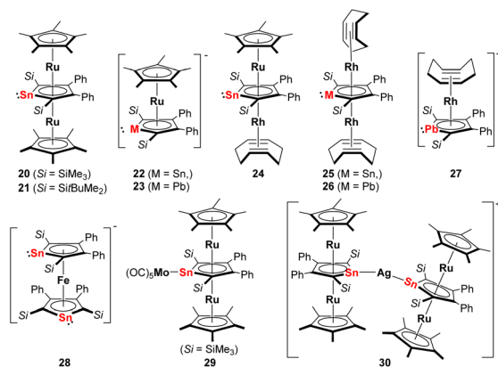
Fig. 4 Late transition metal complexes with \eta^5 -coordinating dianionic stannoles or plumbolones; Si = Si t BuMe 2 , unless otherwise specified. 22–27
