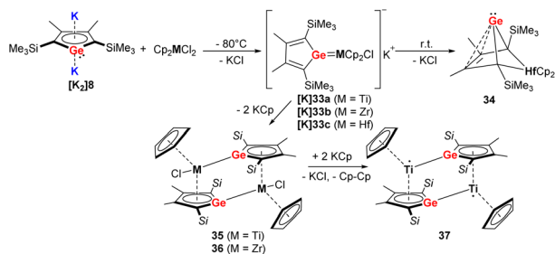
Scheme 6 Reaction of Müller's dipotassiogermole [\text{K}_2]\text{8} towards group 4 metallocene dichlorides. 35,36
