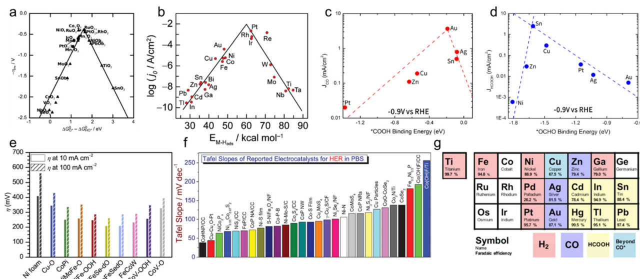
Fig. 4 Volcano plots and catalytic activity of electrocatalysts for different electrochemical reactions. (a) Volcano plot for the oxygen evolution reaction (OER) as a function of the standard free energy. Reproduced from ref. 58. Copyright 2011 Wiley. (b) Volcano plot for the hydrogen evolution reaction (HER) as a function of M-H bonding energy. Reproduced from ref. 71. Copyright 2010 American Chemical Society. Volcano plots for the CO 2 reduction reaction (CRR) to (c) CO using \Delta G_{\text{COOH}} binding energy and (d) HCOO - using \Delta G_{\text{OCHO}} binding energy. Reproduced from ref. 78. Copyright 2017 American Chemical Society. (e) Overpotentials of OER catalysts on Ni foam (NF) in 1 M KOH. Reproduced from ref. 70. Copyright 2021 Cell Press. (f) Tafel slopes of HER catalysts in PBS solution. Reproduced from ref. 72. Copyright 2020 Wiley. (g) Major product classification of metal catalysts for CRR from experiments by Hori. Reproduced from ref. 80. Copyright 2017 Wiley.
