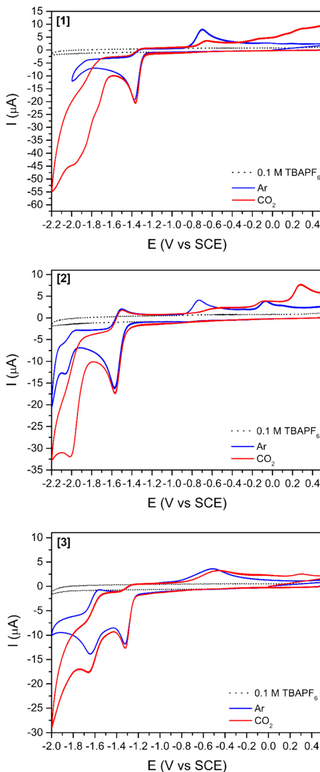
Fig. 2 Cyclic voltammograms of complexes [1], [2], and [3] (1 mM) in DMF, argon, or carbon dioxide saturated solutions using TBAPF 6 as supporting electrolyte (0.1 M) at 100 mV s -1 . Glassy carbon (3 mm diameter) was used as working, platinum wire as counter and SCE as reference electrodes.
